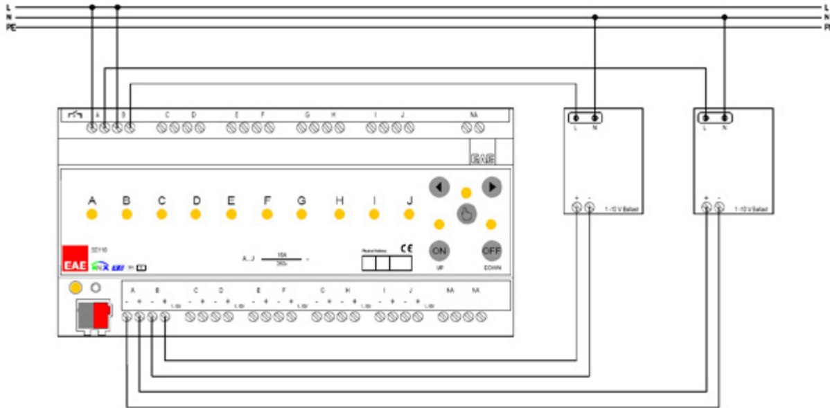
Connection Diagram
